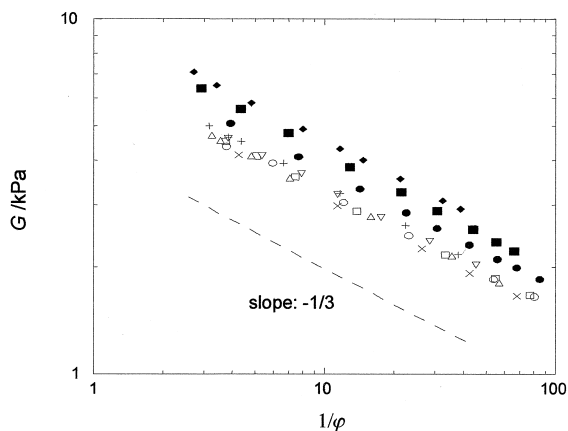
Fig. 2: Variation of the shear modulus G as a function of the swelling ratio 1/\phi . Open symbols: gels swollen in 40 mM NaCl solutions containing different amounts of \text{CaCl}_2 (0–0.8 mM). Closed symbols: gels in 40 mM NaCl solutions containing \text{CoCl}_2 (0.1–0.3 mM).
